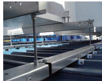
◀ Pier Cover Plate Mounting
